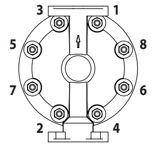
Torque Sequence
