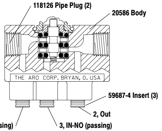
Model 2( )(-C 5/32" Tubing Ports
