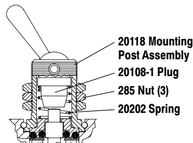
Model 223-C & 223-2-C Retained Toggle
