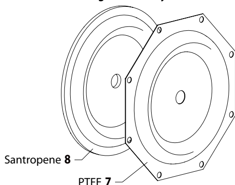
View for PH20F-XXX-XXT-C (PTFE diaphragm) configuration only.
