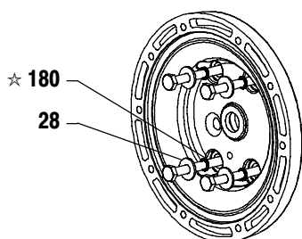
AUXILIARY VIEW A-A (models PX15R-XXX-XXX)
